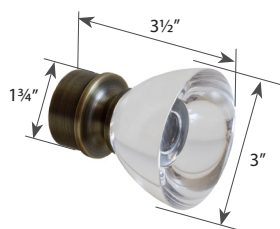
INFINITY GLASS FINIAL BRUSHED GOLD COLLAR DSG01/BGO
