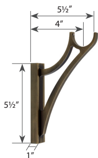
METAL BRACKET DSG42/BGO
