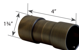
SPLICE SLEEVE DSG50/BGO
