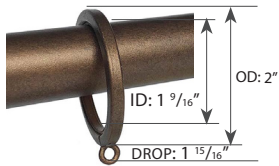
RING COPPER DFR30/COP
